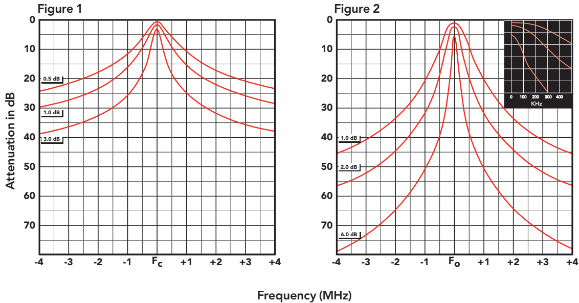
TYPICAL BANDPASS CAVITY RESPONSE CURVES
