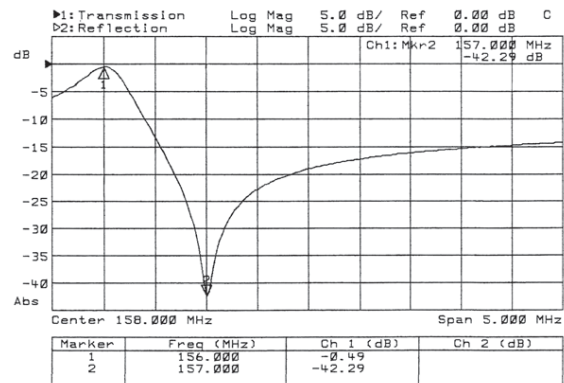
Figure 2 TPRC-1510-1 0.5 dB INSERTION LOSS 1 MHz PASS TO REJECT
