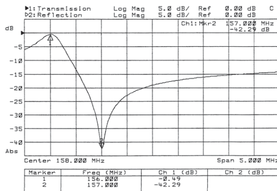
Figure 2 TPRC-1510-1 0.5 dB INSERTION LOSS 1 MHz PASS TO REJECT
