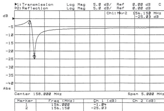
Figure 1 TPRC-1510-1 1 dB INSERTION LOSS 150 kHz PASS TO REJECT
