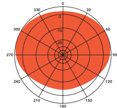
H-Plane gain 8.5dBd 3/8 wl. spacing from tower
