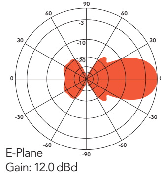
ANT2350Y12-WR at 2400 MHz
