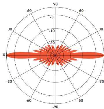
Vertical Plane Gain = 8 dBd Antenna Pattern available on website
